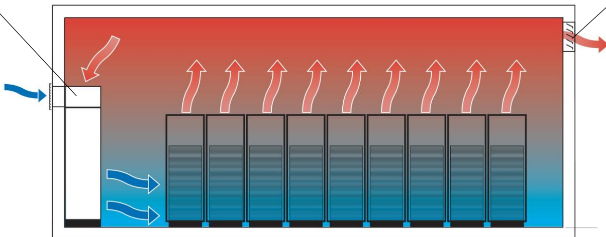
FREE-COOLING plenum
